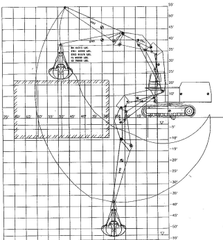
EXISTING LAYOUT WITH FUNCTIONAL ORIGINAL STICK AS IS 1/2" #82-ON STICK (ORIGINAL STICK REQUIRES STICK CYLINDER & LEVEL CYLINDER) PROPOSAL #2 (WITH LOADED BOOM PROFILE)
